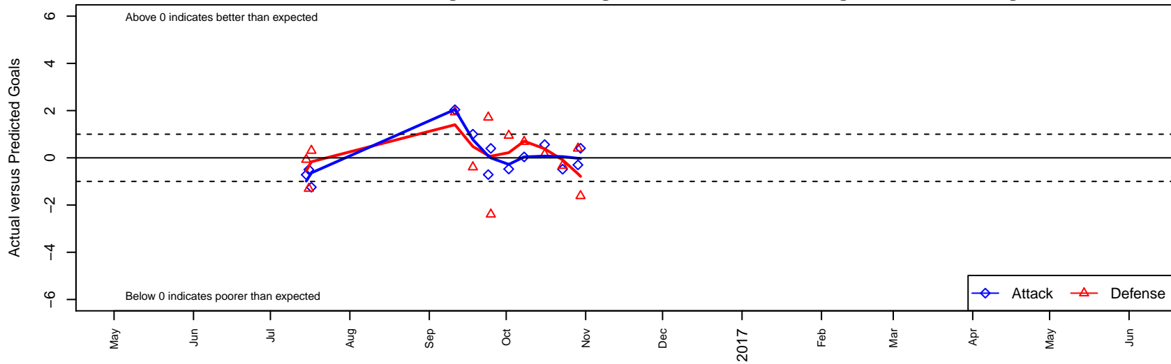
Pateadores Irvine B01 Dots are actual minus expected GF (blue circles) and GA (red triangles). Blue line is smoothed change in attack strength. Red is smoothed change in defense strength.
